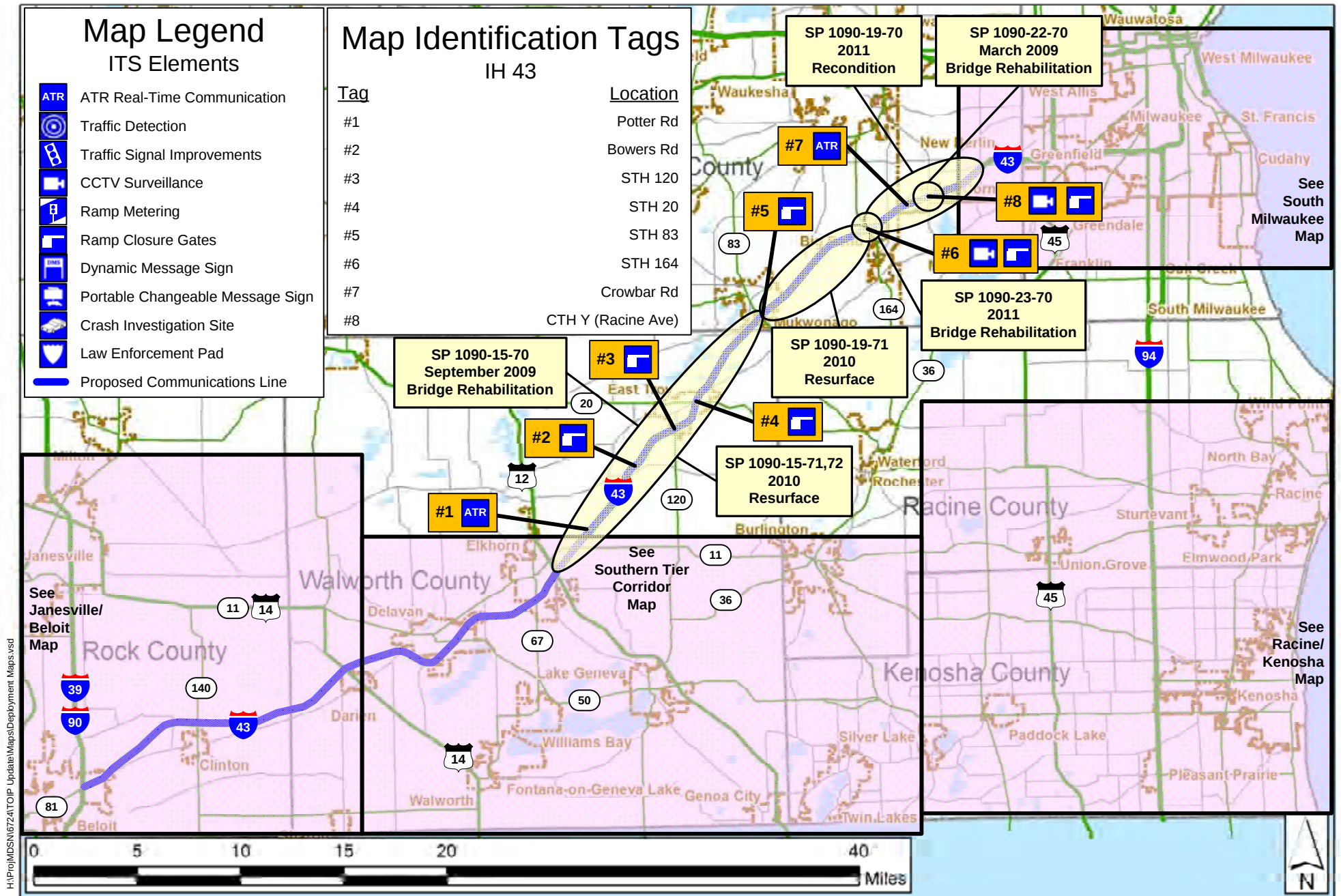
Glacial Plains Corridor – TOIP Based ITS Deployment
